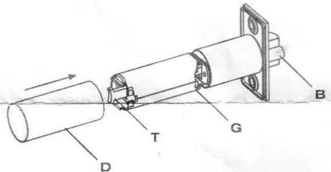
Fig. 2 Check the clearance "G" is in the same side as dead locking pin "B" after assembly.
