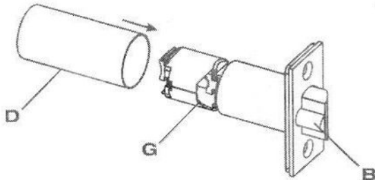
Fig. 4 Assemble sleeve "D" to hold both latch and latch extension.
