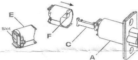
Fig. 3 After assembly, clearance "G" to be in the same side as dead locking pin "B".
