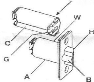
Fig. 2 Check the clearance "G" is in the same side as dead locking pin "B" after assembly.
