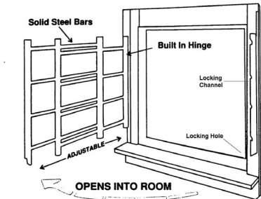
Window Guard Dimensions 1130 SERIES
