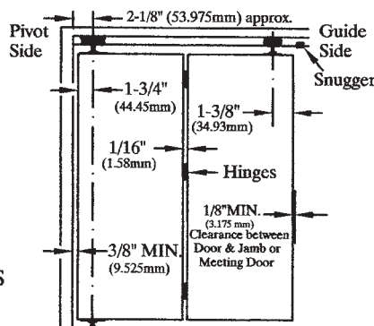
Fig. 1 2 OR 4 PANEL BI-FOLD
