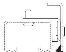
3126 Sidewall Bracket
