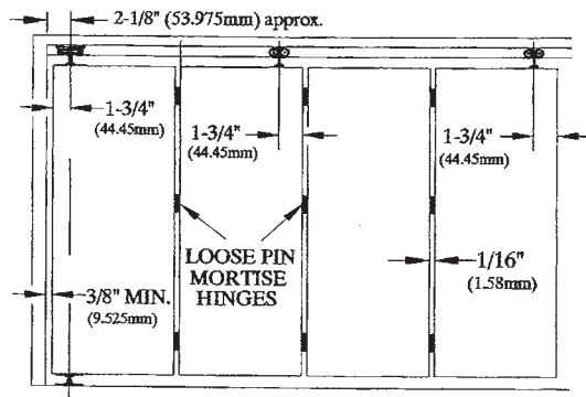
Fig. 2 MULTI-FOLD
