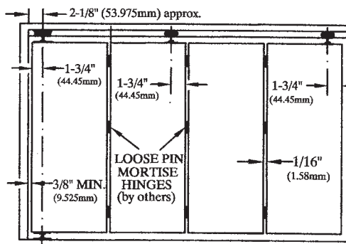
Fig. 2 MULTI-FOLD
