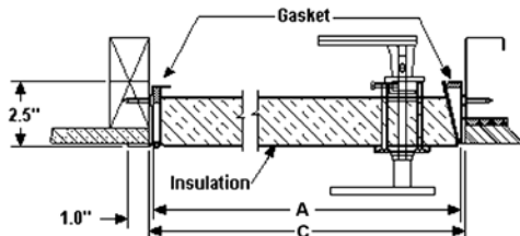
Door Sizes and Wall Openings: Models XPA, XPS, XPA-PWE, AND XPS-PWE
