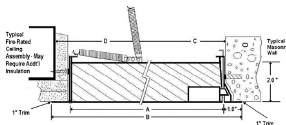
Ceiling Installation - FD-FDSS-HGFD Side View
