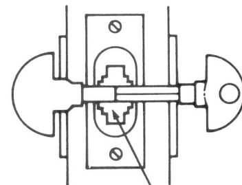
SPINDLE CUT TO ENGAGE HALF-WAY IN HUB
