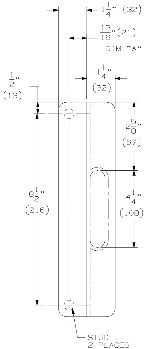
LG10 OVERALL SIZE 2 1/2" X 9 1/2"
