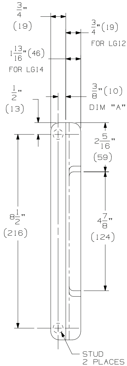
LG12 & LG 14 LG12 OVERALL SIZE 1 1/2" X 9 1/2" LG14 OVERALL SIZE 2 9/16" X 9 1/2"
