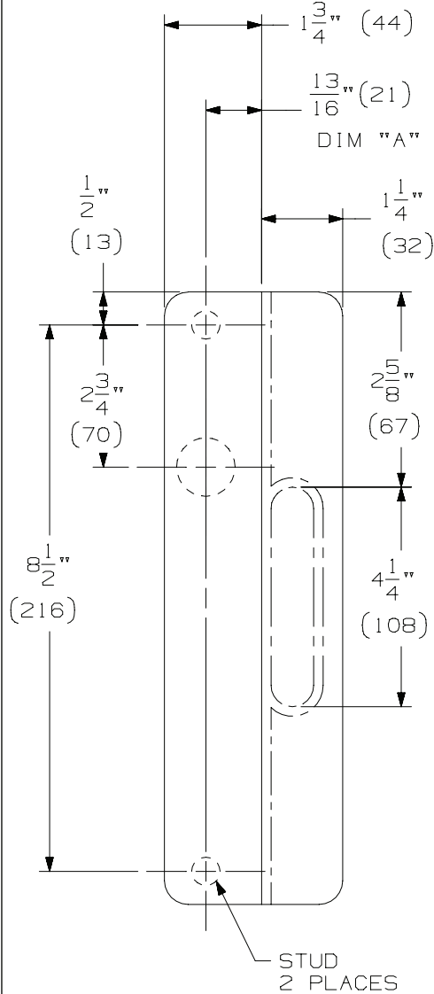
LG11 OVERALL SIZE 3" X 9 1/2"
