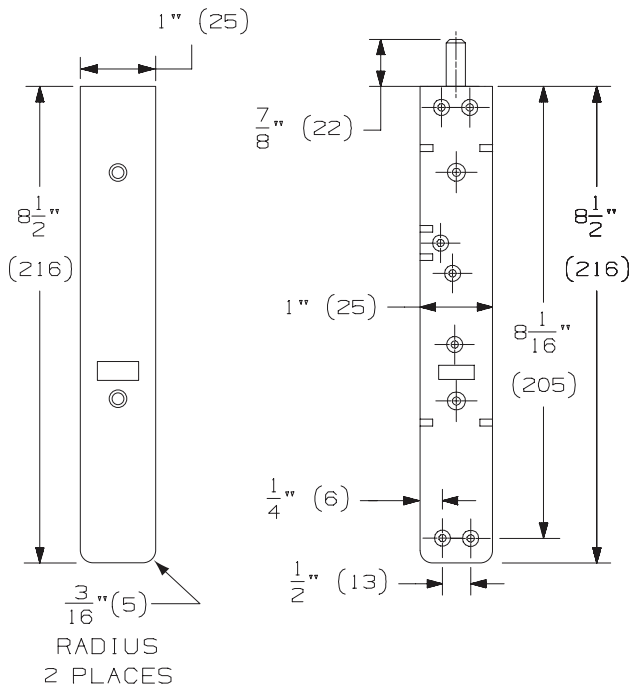
FB41T & FB41B BASIC PART DIMENSIONS
