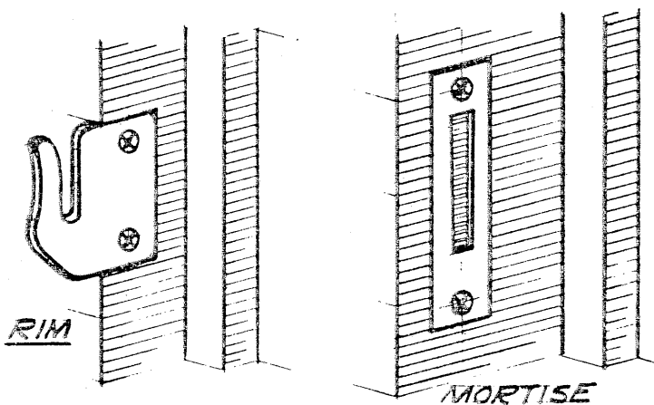
MORTISE STRIKE
