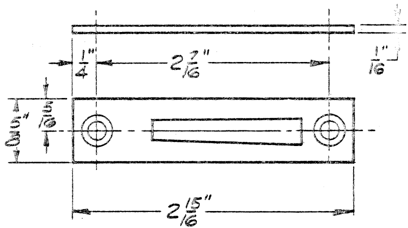
MORTISE STRIKE
