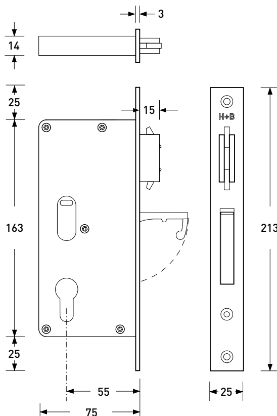
Lock body
