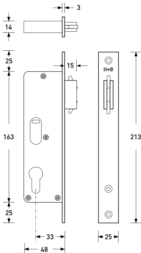
Lock body
