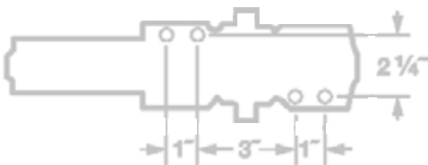
Hole Pattern
