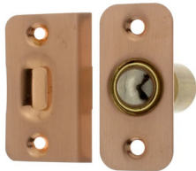
#12012 Wide Round Roller Ball Catch Face: 1" x 2-1/8" Strike: 1-3/8" x 2-1/8" Tube Diameter: 3/4" Tube Length: 1 1/2"
