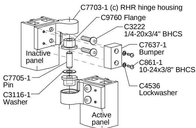
C7702-1 RHR hinge assembly for RHR &amp; LH units
