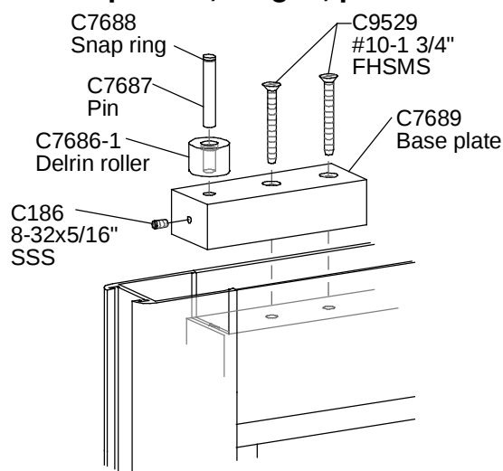
Top roller guide for inactive panel
