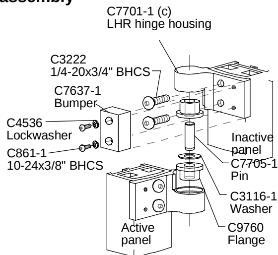
C7700-1 LHR hinge assembly for LHR &amp; RH units
