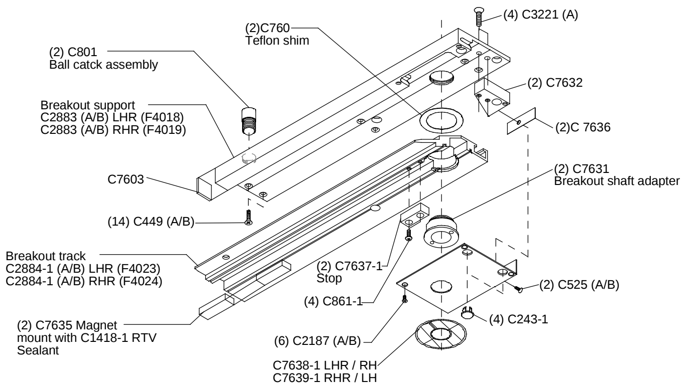
C7618 Bifold breakout assembly for pair units (half shown) C7619 &amp; C7620 similar.
