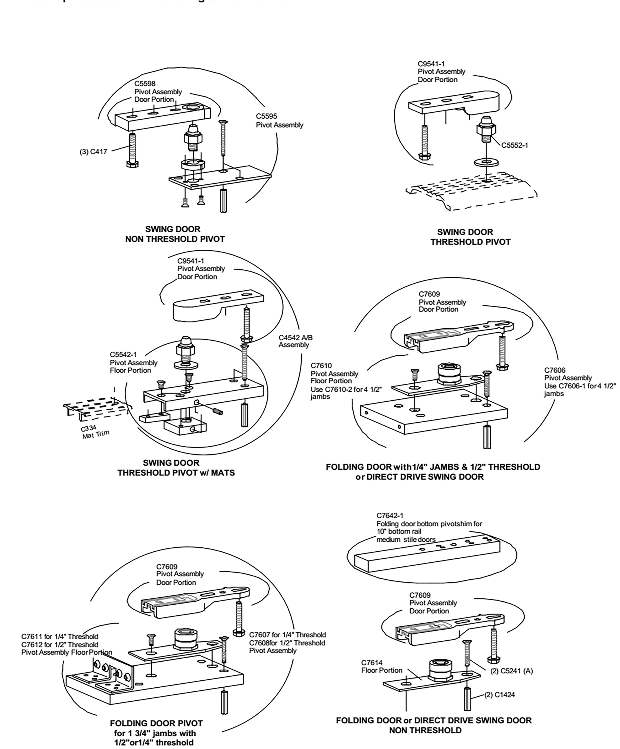
Bottom pivot assemblies for swing & bifold doors
