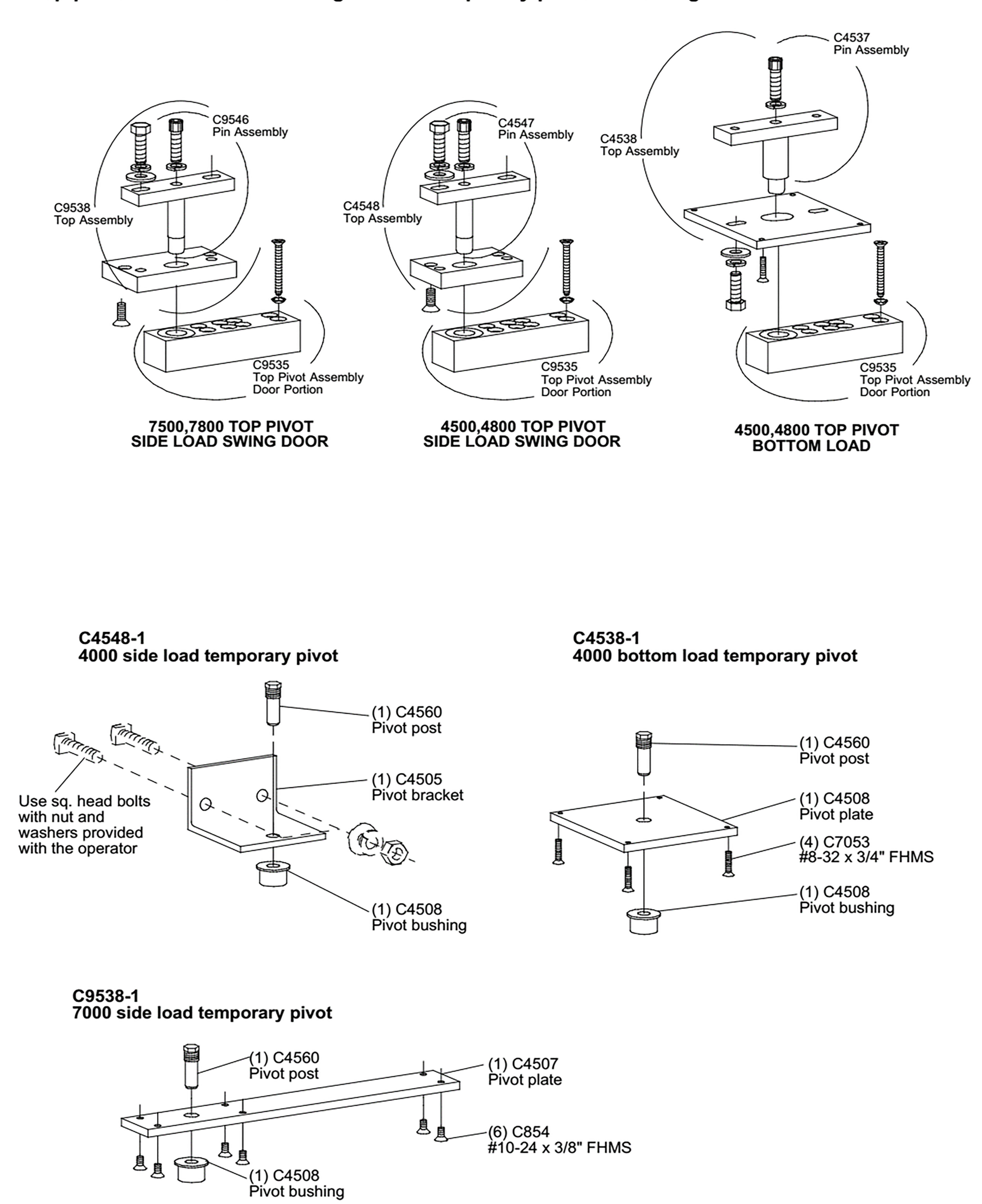
Top pivot assemblies for swing doors. Temporary pivots for swing doors
