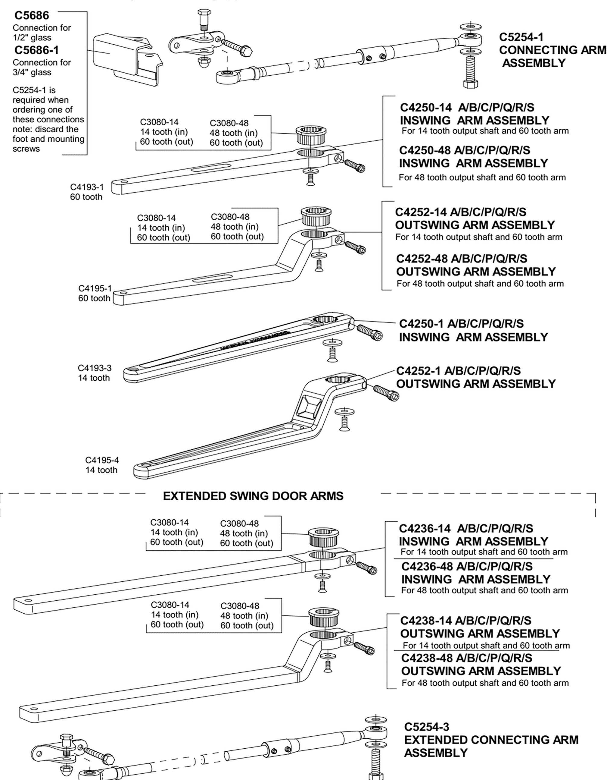
Arm assemblies swing door & folding applications
