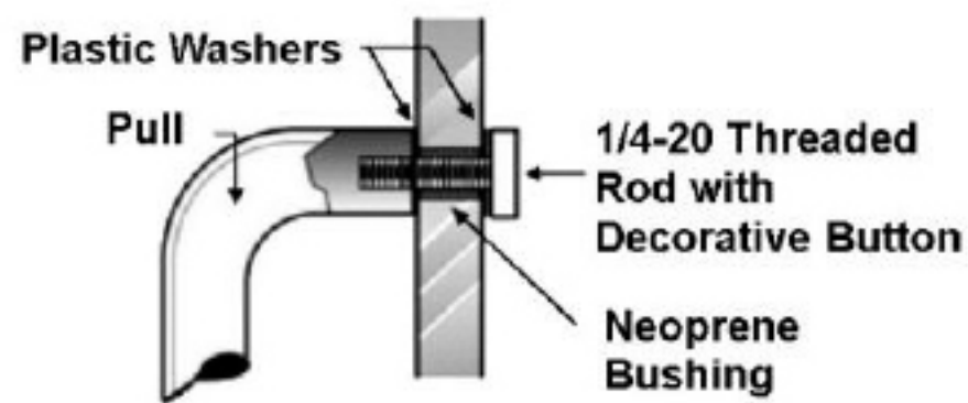
Decorative Thru-Bolt - .A5
