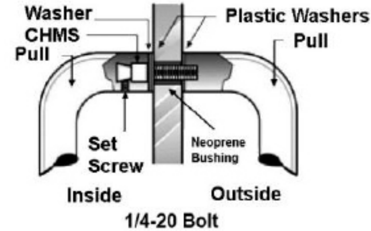
Back-to-Back Pull/Pull - .GS5
