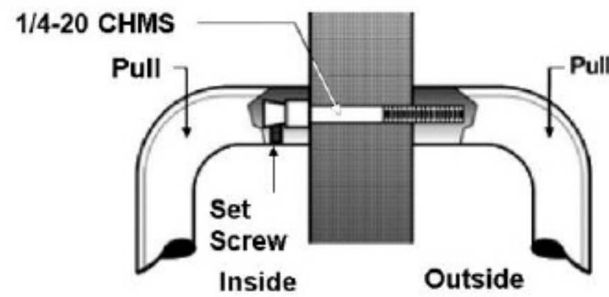
Back-to-Back for Pull/Pull - .WS Minimum Pull Dia. 5/8"
