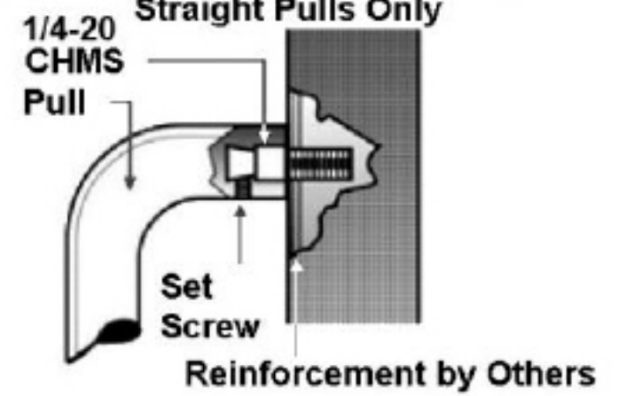
Surface Concealed - .SM Metal Door - Minimum Pull Dia. 5/8" Straight Pulls Only
