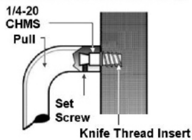
Surface Concealed - .SW Wood Door - Minimum Pull Dia. 5/8"
