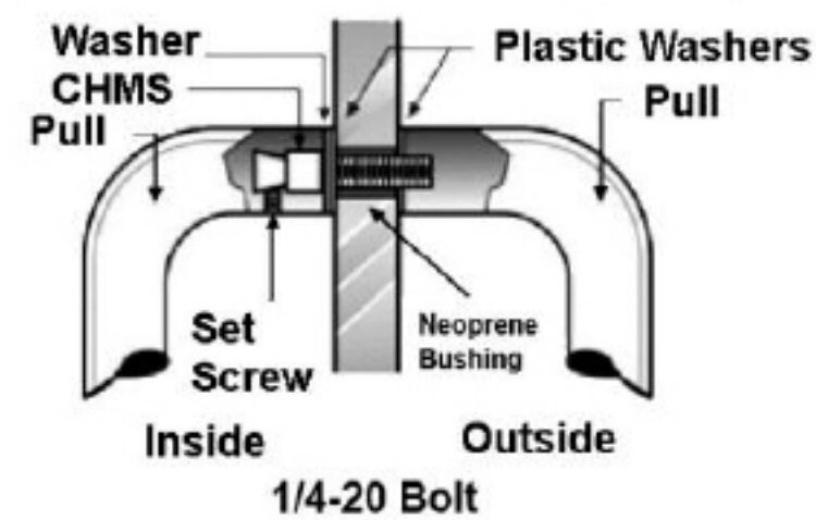
Back-to-Back Pull/Pull - .GS5
