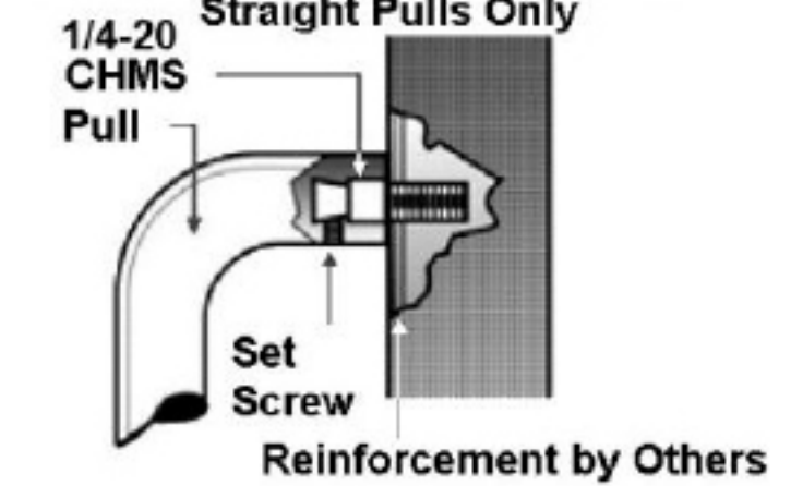
Surface Concealed - .SM
