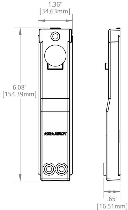
Mounting Bracket
