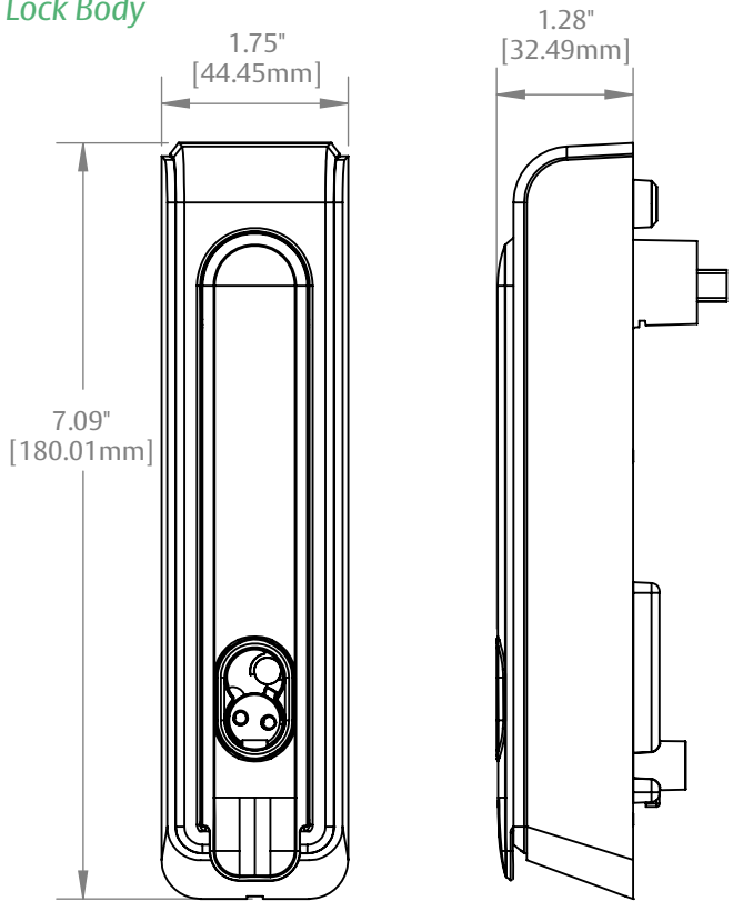
Lock Body
