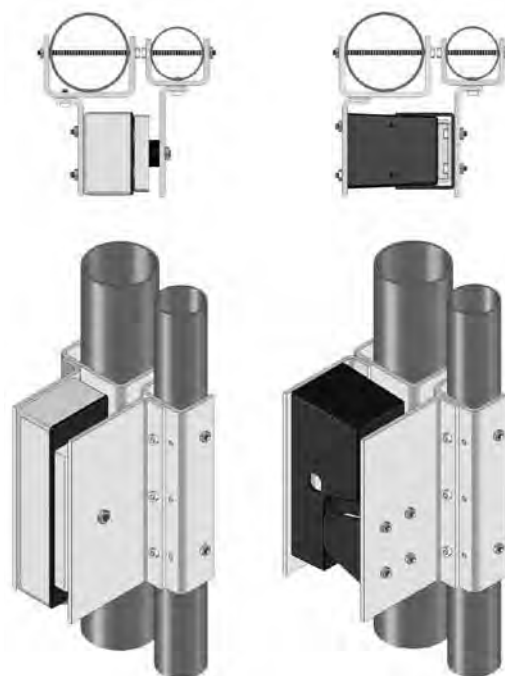
Securitron FMK-SL shown with Securitron M62FG
