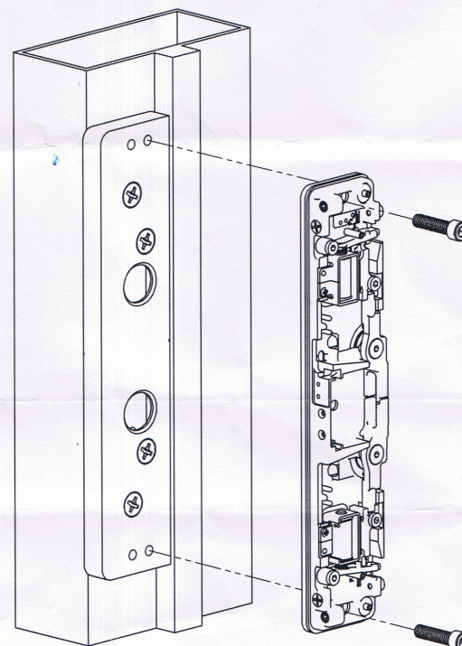
Diagram 2 Installing Product
