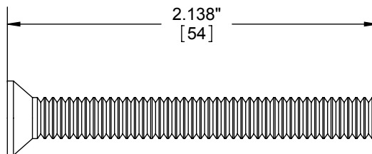
1/4-20 FLAT PHILLIPS HEAD MACHINE SCREW (#3 HEAD)
