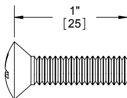
1/4-20 OVAL PHILLIPS HEAD MACHINE SCREW (#3 HEAD)
