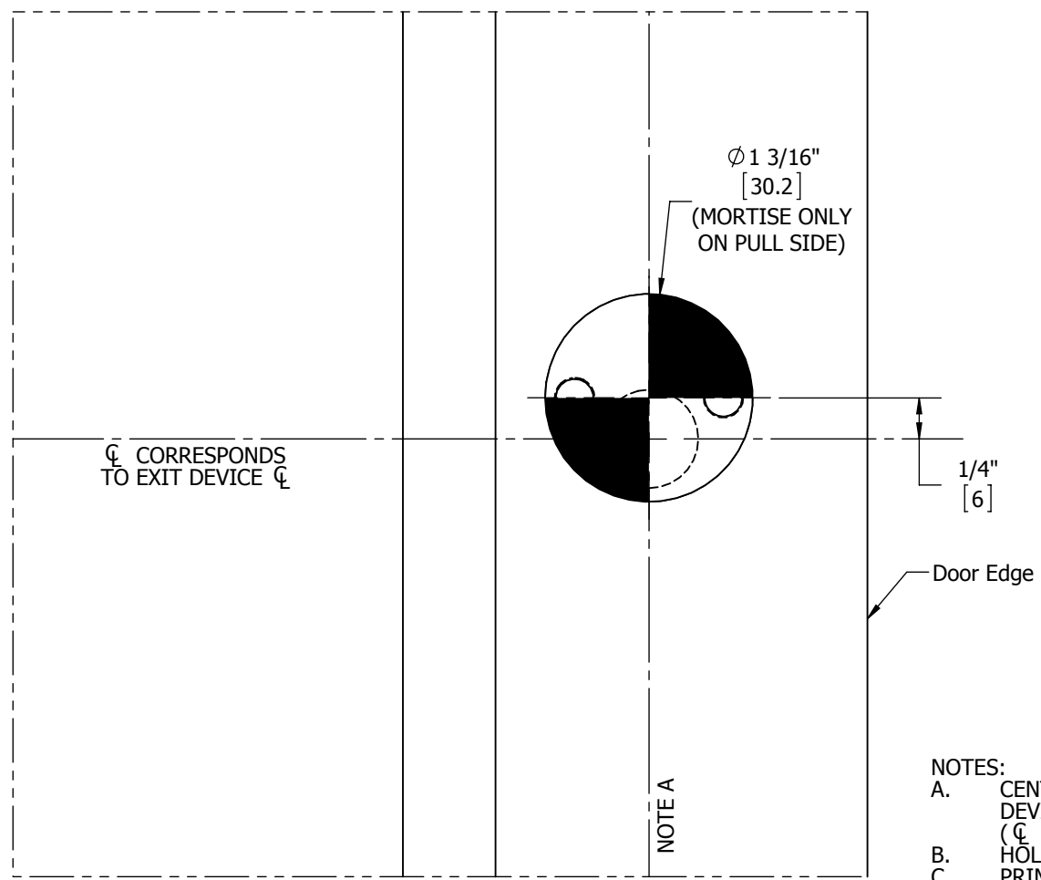
PULL SIDE OF DOOR (RIM CYLINDER IS MOUNTED ON THIS SIDE)
