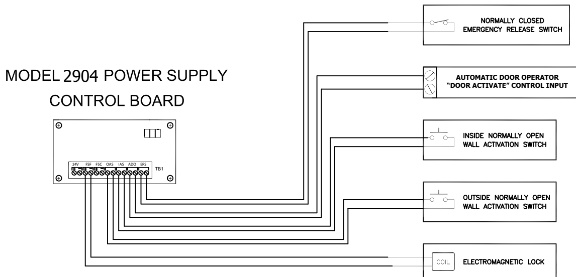
POINT-TO-POINT WIRE DIAGRAM FOR AUTOMATED DOOR OPENING SYSTEM APPLICATION USING AN ELECTROMAGNETIC LOCK
