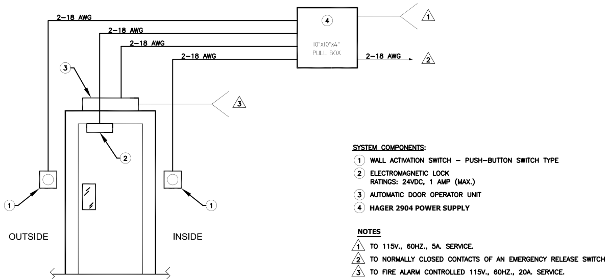
RISER DIAGRAM FOR AUTOMATED DOOR OPENING SYSTEM APPLICATION USING AN ELECTROMAGNETIC LOCK
