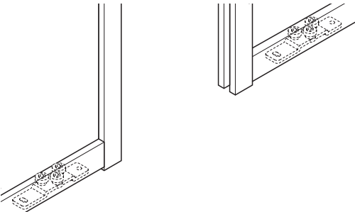
Lower guide without guide channel
