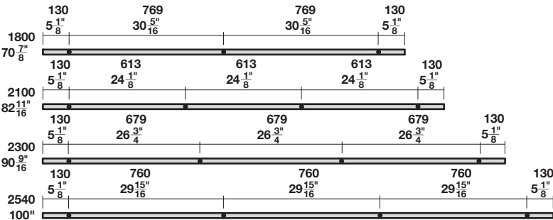
Drilling dimensions for solid tube upper tracks:
