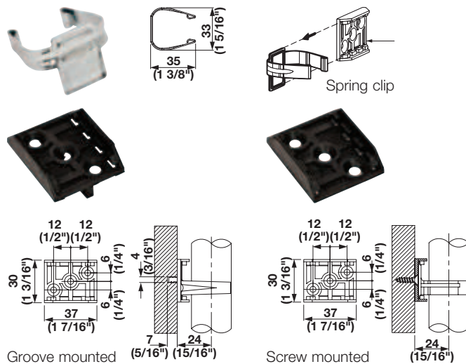
Groove mounted
