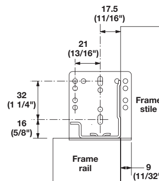
Rear Bracket Position
