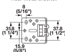
Rear metal bracket
