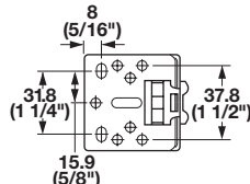
Rear metal bracket
