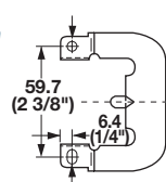
Front clip-on bracket
