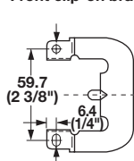
Front clip-on bracket
