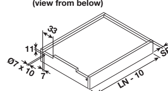
Drawer drilling (view from below)
