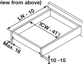
Drawer with front (view from above)
