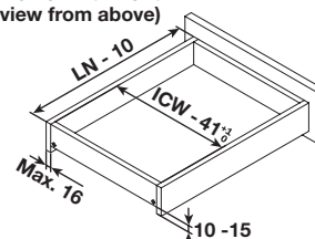
Drawer with front (view from above)
