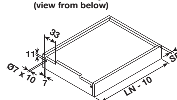
Drawer drilling (view from below)
