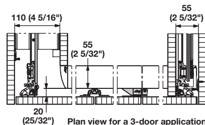
Plan view for a 3-door application
