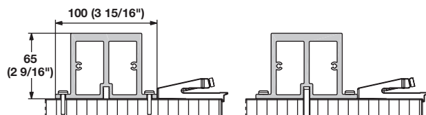
Profile, pre-assembled
