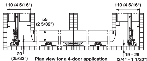
Plan view for a 4-door application
