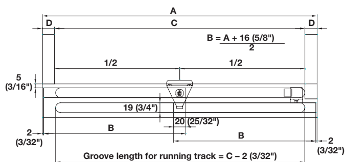
Drilling pattern
