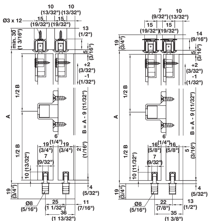
Mounting example with 19 mm (3/4") door and track 405.87.082.
