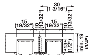
Double upper track, screw mounted
