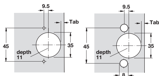
Screw mount
