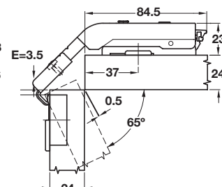
24 mm door thickness Mounting plate height 0 mm
