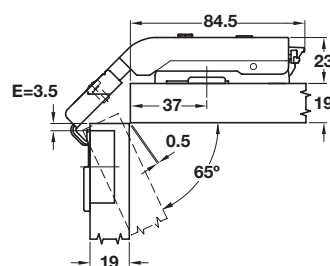
19 mm door thickness Mounting plate height 0 mm
