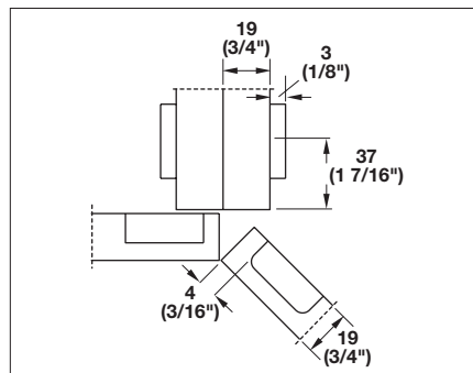
Concealed hinge 329.96.507 / page 9.27 Mounting plate 329.71.110 / page 9.38
