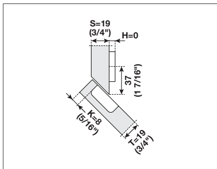
Concealed hinge 329.25.448 / page 9.27
