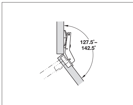
Concealed hinge 329.96.507 / page 9.27 Mounting plate 329.84.110 / page 9.42
