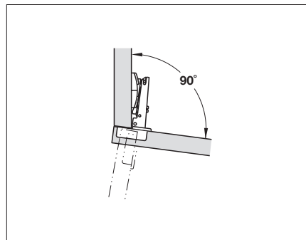
Concealed hinge 329.28.500 / page 9.18 Mounting plate 329.84.110 / page 9.42
