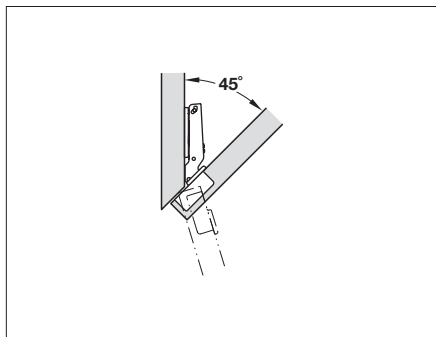
Concealed hinge 329.09.591 / page 9.27 Mounting plate 329.71.500 / page 9.38
