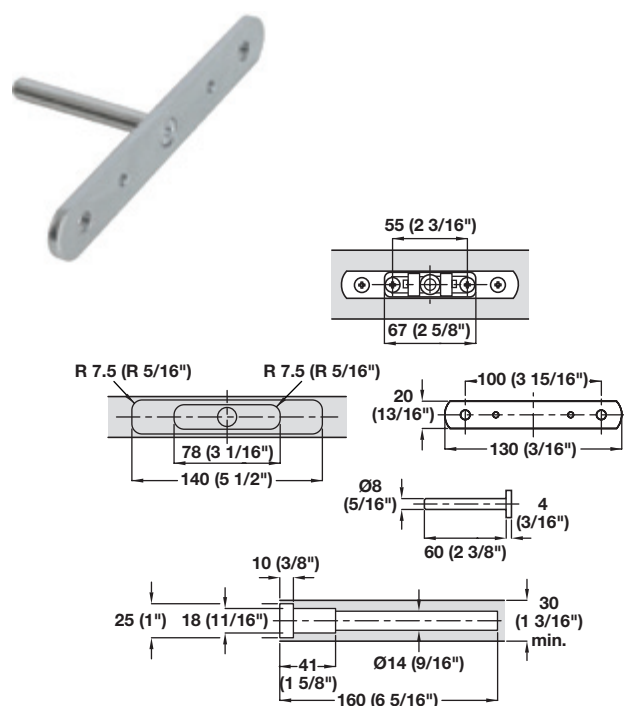
→ TRIADE Shelf Support - Bracket
