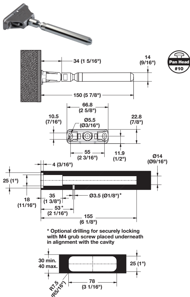
→ TRIADE Shelf Support
