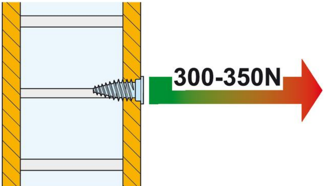
Lightweight panel with 4 mm thin chipboard top layer
