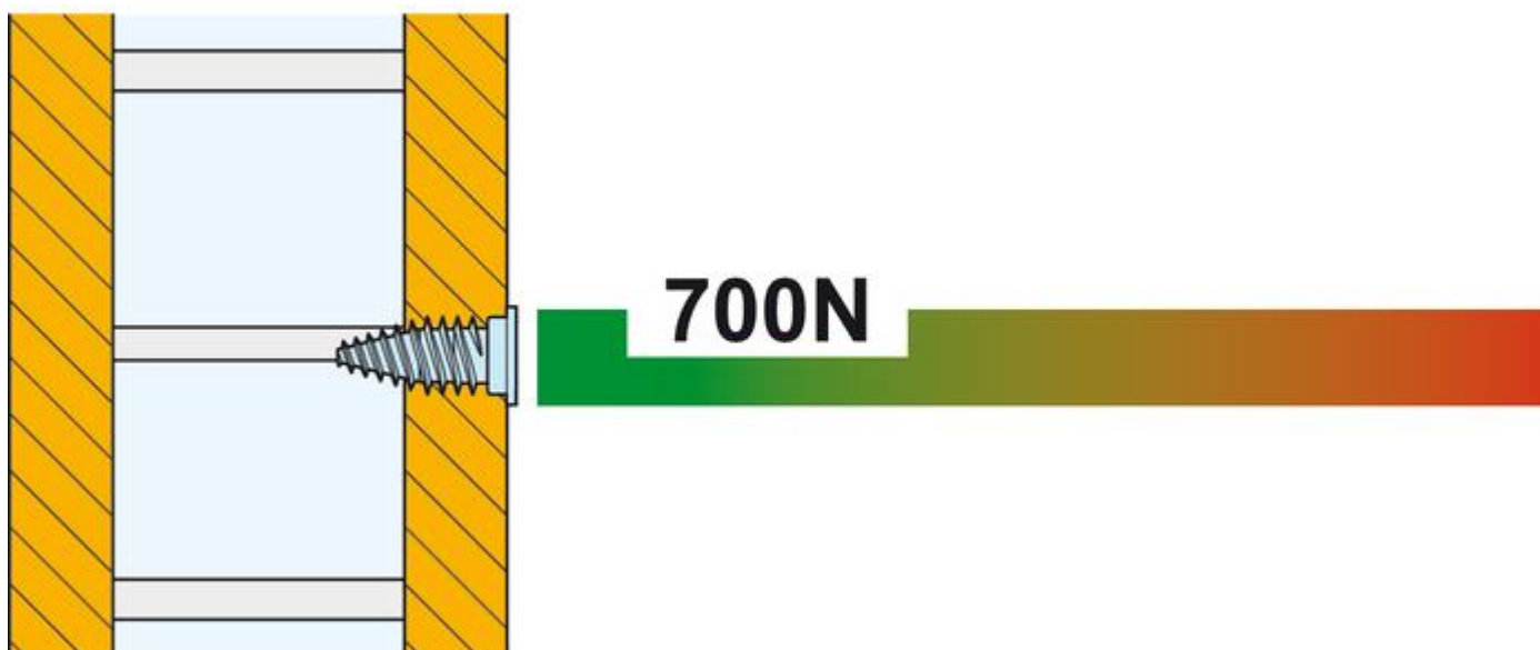
Lightweight panel with 8 mm thin chipboard top layer
