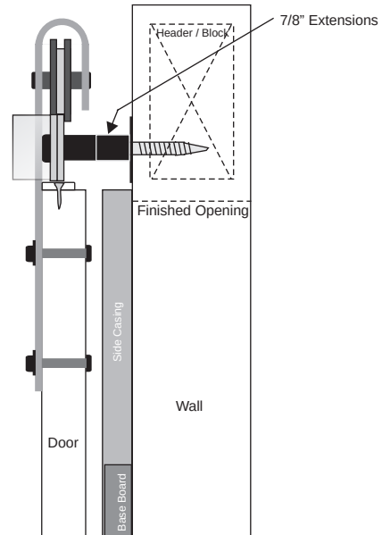
Std Hardware Pack + 7/8" Extension Kit installed where casing, base, or other trim, is 5/8" to 1" thick .
