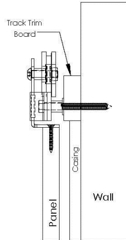
Std Hardware Pack installed on track trim board that is equal to or thicker than casing or other trim
