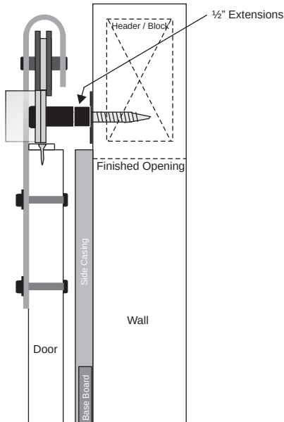
Std Hardware Pack + 1/2" Extension Kit installed where casing, base, or other trim, is up to 1/2" thick .
