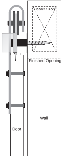
Std Hardware Pack installed with no casing, base, or other trim.
