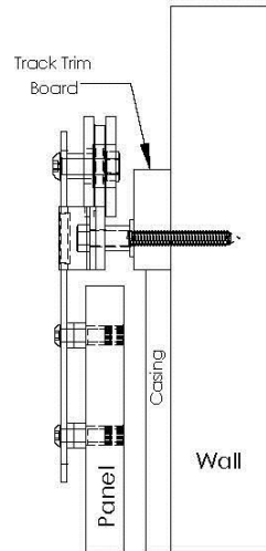
Std Hardware Pack installed on track trim board that is equal to or thicker than casing or other trim
