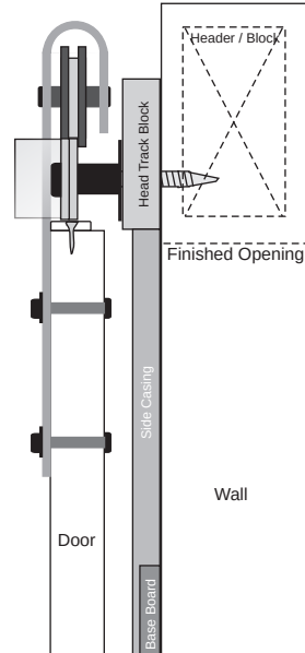
Std Hardware Pack installed on track trim board that is equal or thicker than casing, base, or other trim.
