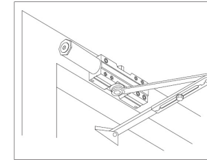
MOUNTED OVER DOOR FACE ( PUSH SIDE )
