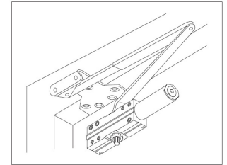
MOUNTED ON STOP FACE ( PUSH SIDE ) PARALLEL ARM
