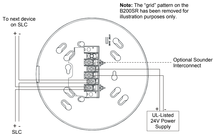
Figure 9.4 Wiring of a B200SR Sounder Base
