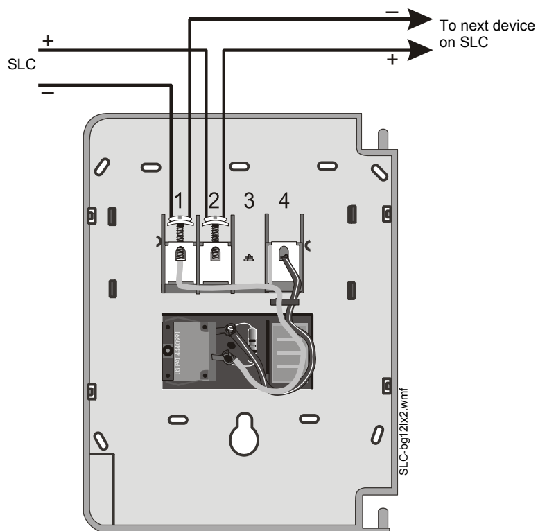
Figure 10.1 Wiring of a BG-12LX Pull Station to an SLC
