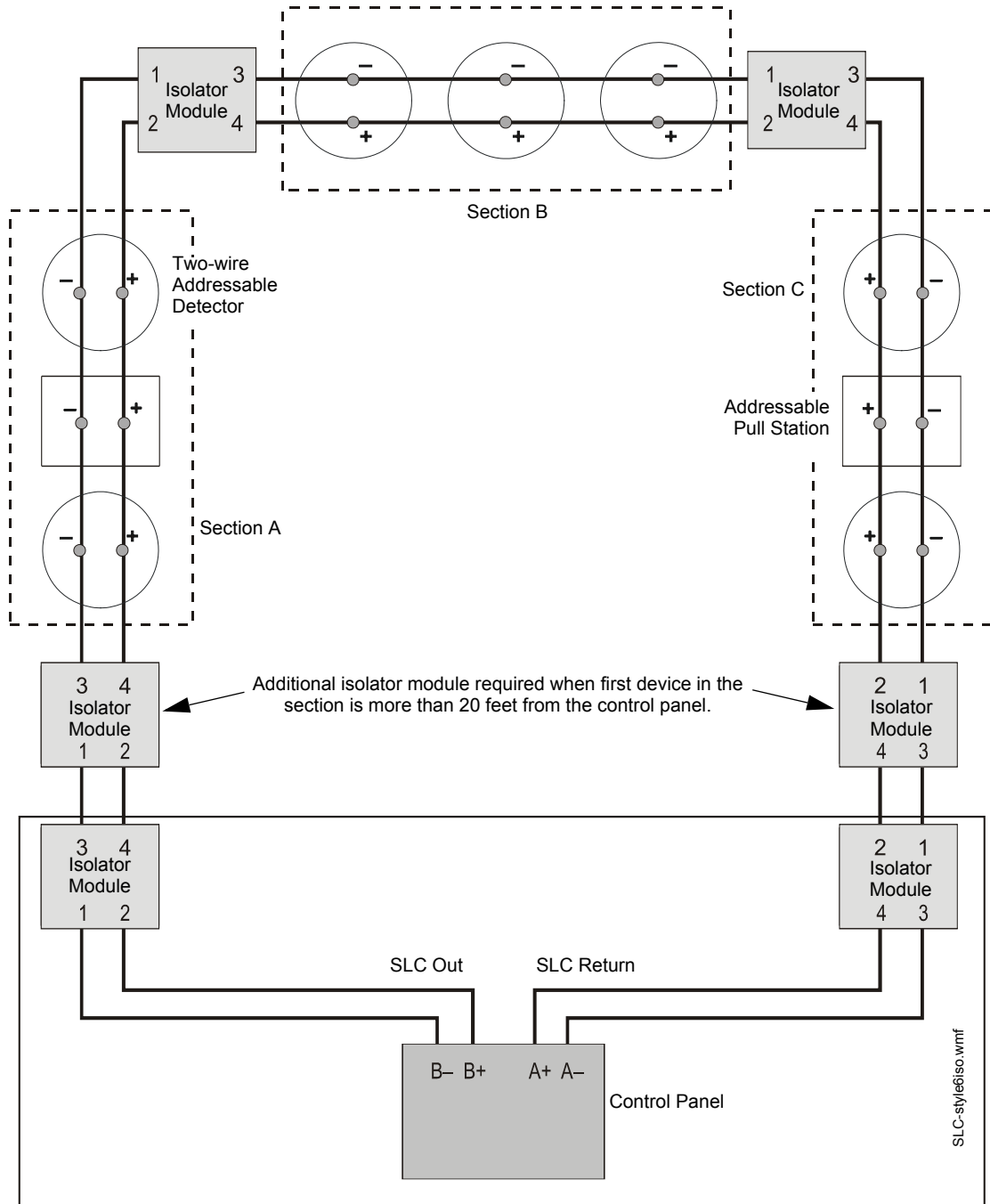
Figure 4.3 NFPA Style 6 SLC Using Isolator Modules
