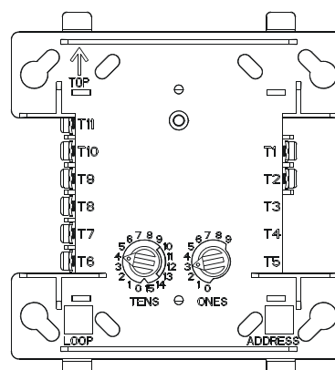
CMF-300 Newer Version Module (Horizontal Rotary Dial)
