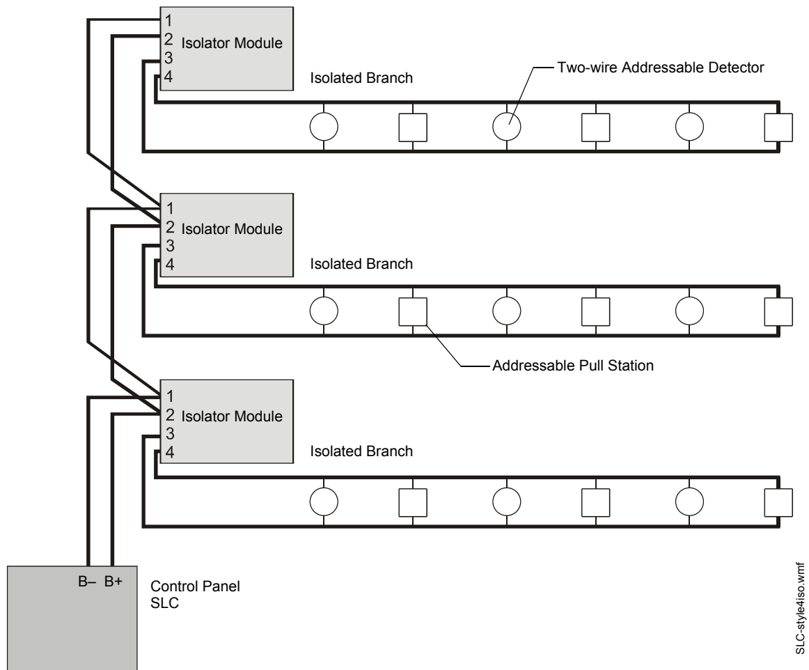
Figure 4.2 NFPA Style 4 SLC Using Isolator Modules
