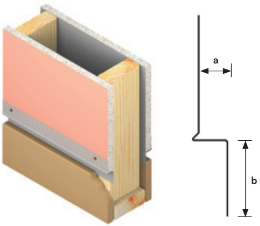
Custom size profile. Please specify sizes when ordering.
