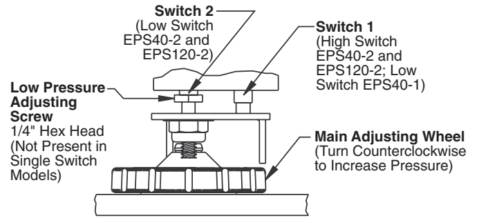
FIGURE 5. ADJUSTMENTS (DUAL-SWITCH MODEL SHOWN):
