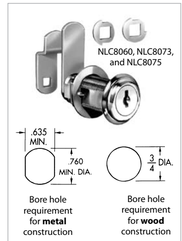
Thick door/drawer construction using NLC8073 with NLC7014-2C cam (sold separately)
