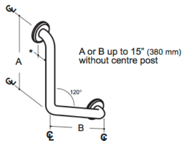
12 120° Angle Bars
