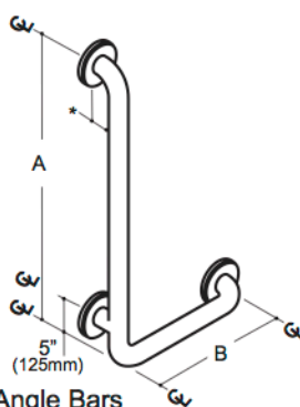
08 90° Angle Bars
