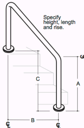
52 Stair Rail
