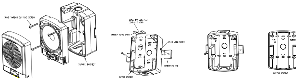
Figure 6 A & B: Surface Backbox Mounting
