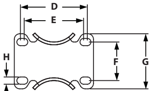
RIGID CASTER
