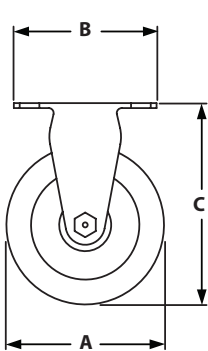
RIGID CASTER
