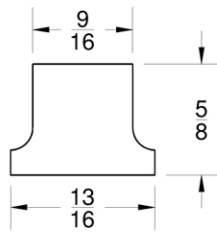
STANDARD DOORLITE MULLION
