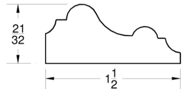
PLANT MLDG #204
