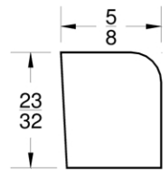
STANDARD FLUSH DOORLITE MOULDING #300
