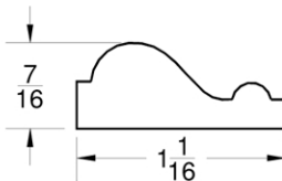
PLANT MLDG #203
