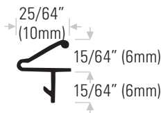
DSPF109T Extruded vinyl/tan. Length available: 12ft (3658mm) only. DSPF109W White
