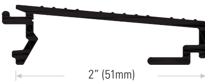
DS1122A150 Extruded aluminum mill finish. Length available: 150" (3810mm) only
