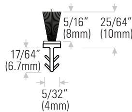
DSP108-35BL 5/16" (8mm) pile height, black
