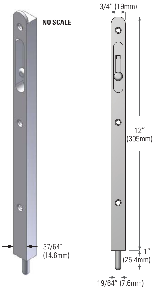
DS14-26D Flushbolt, satin finish DS14-10B bronze
