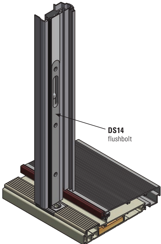
DS14-26D Flushbolt, satin finish DS14-10B bronze
