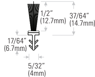
DSP108-50BL 1/2" (12.7mm) pile height, black
