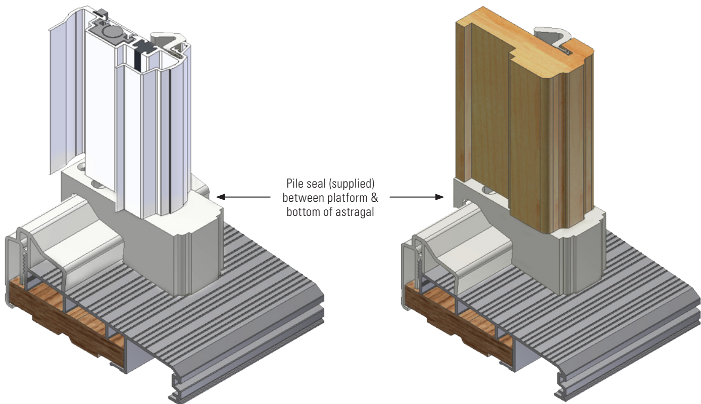
DS346/348 SERIES Aluminum astragal
