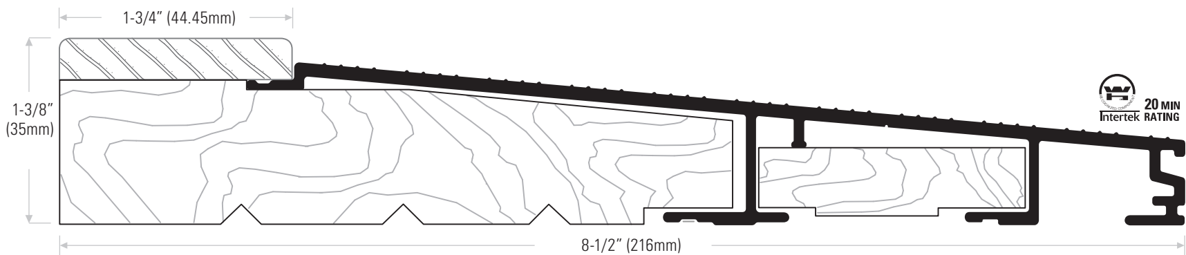
DS814A0AK Extruded aluminum sill, mill finish with fixed oak cap. Length available: 108" (2743mm) only DS814DOAK Bronze anodized with fixed oak cap.
