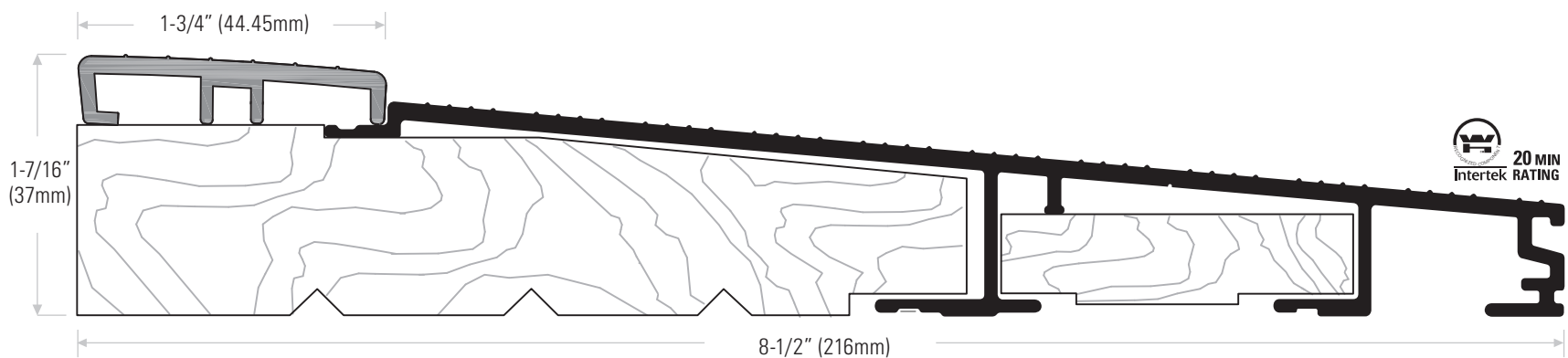
DS814AVT Extruded aluminum sill, mill finish with fixed vinyl cap, tan. Length available: 108" (2743mm) only DS814DVBL Bronze anodized with fixed vinyl cap, black.
