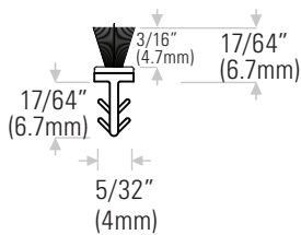
DSP108-20BL 3/16" (4.7mm) pile height, black
