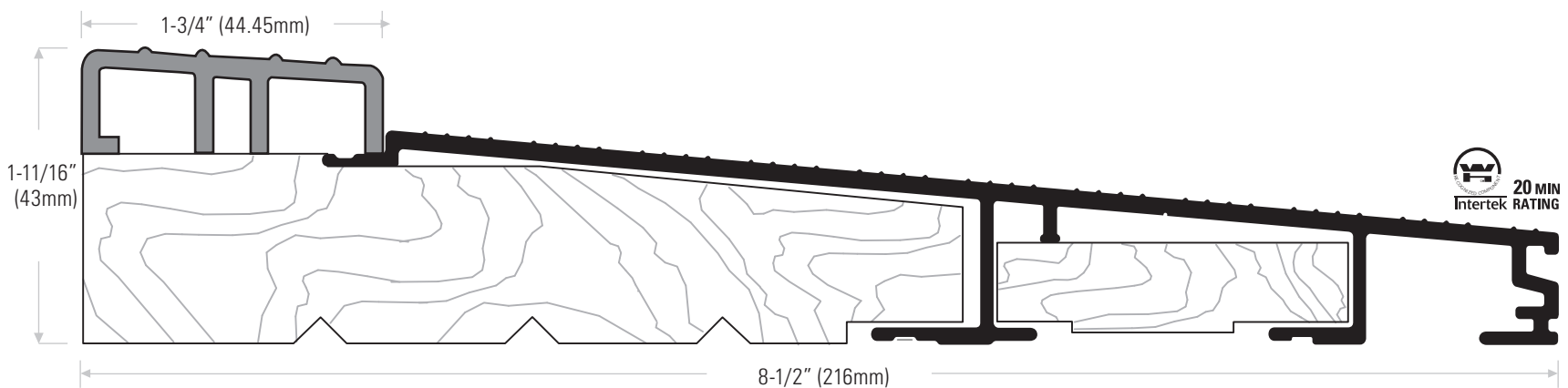
DS814AHVT Extruded aluminum sill, mill finish with fixed high vinyl cap, tan. Length available: 108" (2743mm) only DS814DHVT Bronze anodized with fixed high vinyl cap, tan.
