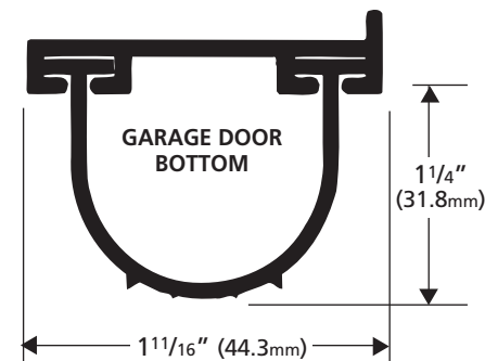
DS208 Extruded Aluminum with cold temperature vinyl insert Grey DSV08GREY Vinyl Insert Only - Grey
