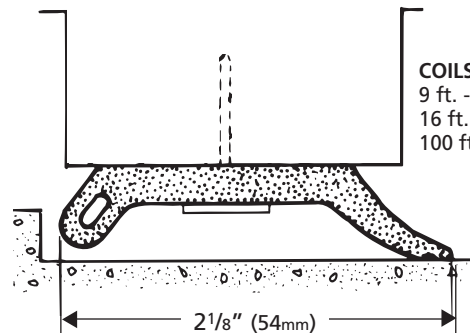
DS37BL Extruded Black Sponge Neoprene DS37BL9 9ft. - 2.74m DS37BL16 16ft.- 4.87m DS37BL100 100ft. - 30.4m
