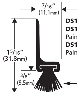
DSP12GREY Grey Pile Replacement Insert
