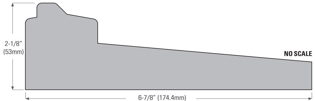
DS658SGASKET Adhesive backed sill end gasket 6-5/8" (168mm) wide for 4-5/8" and 6-5/8" sill, trim to suit.
